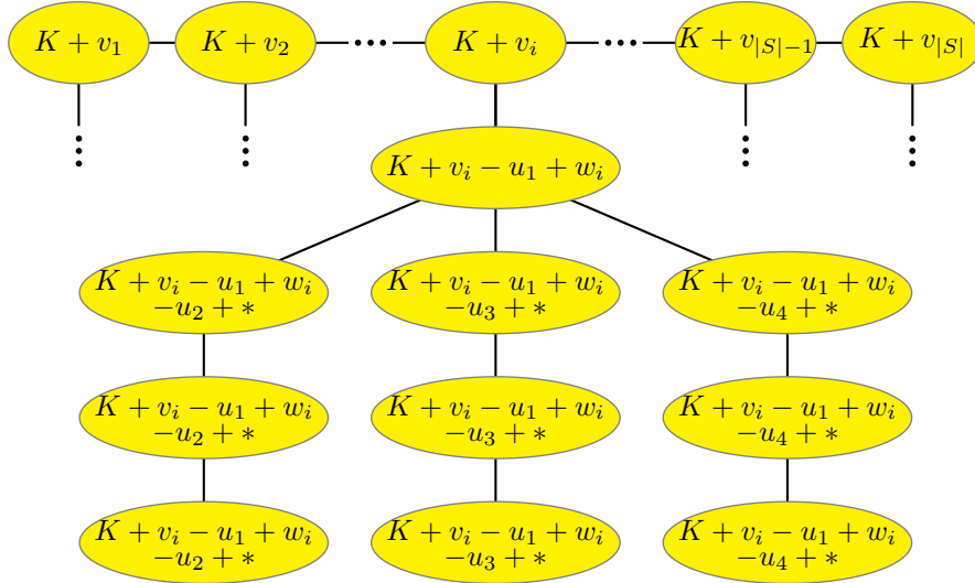
Figure 2: A smooth degree-4 tree decomposition of Q .
