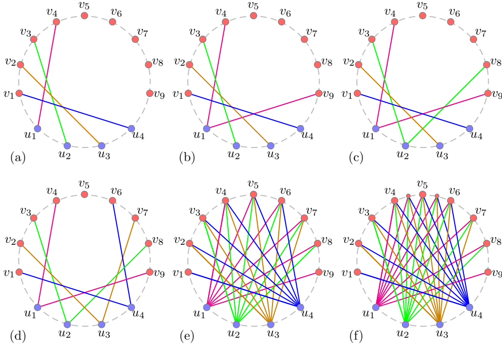
Figure 3: Illustration of the proof of Theorem 1 with k = 4 .
