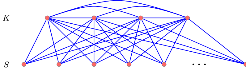
Figure 1: The complete split graph K_{4,|S|^*} .
