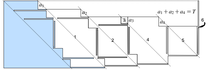
Figure 4. The reduction from a positive instance of SUBSET SUM to an orthogonal polygon (shaded), and a sequence of flipturns that leads to an orthogonal pocket.
