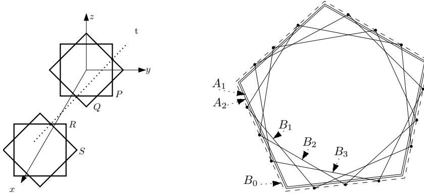
FIG. 4.1. Lower bound examples for Lemmas 4.1 and 4.2.
