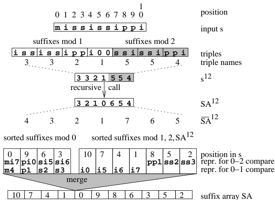
Fig. 1. The skew algorithm applied to s = mississippi .
