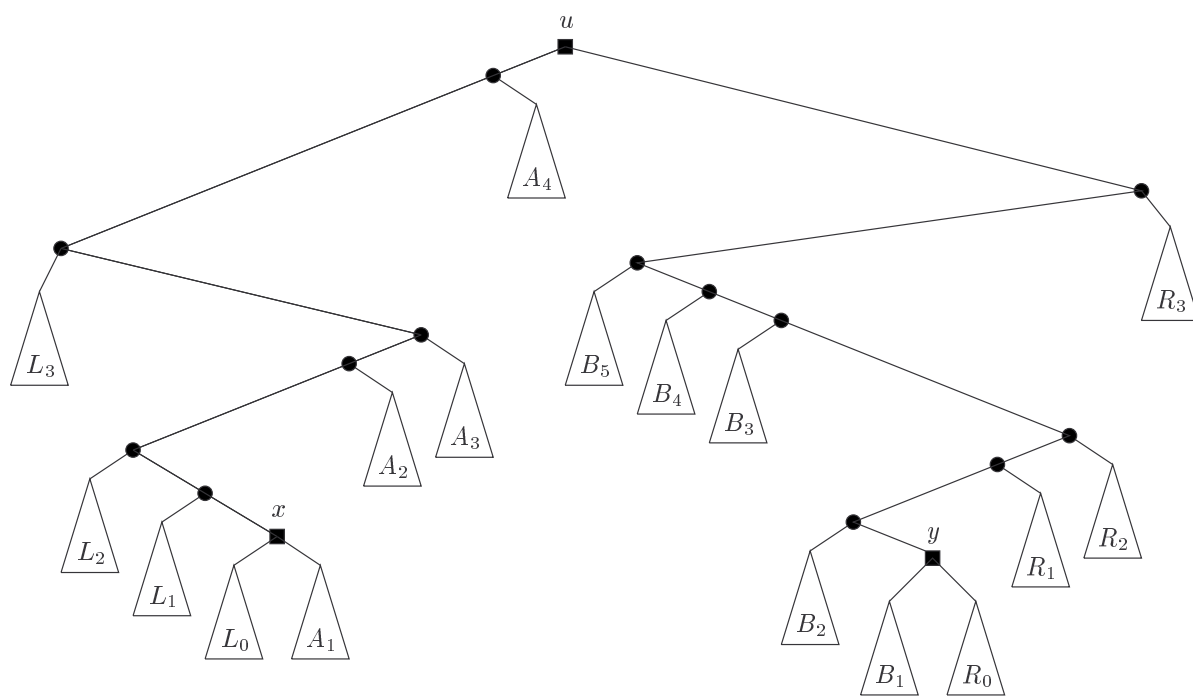
Figure 4: Subtree T_u before the excision
