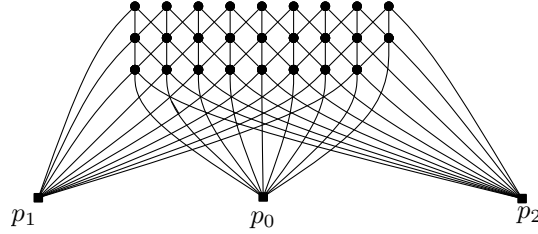
Fig. 4. The graph G for a set of points with i = 9 and t = 3 .
