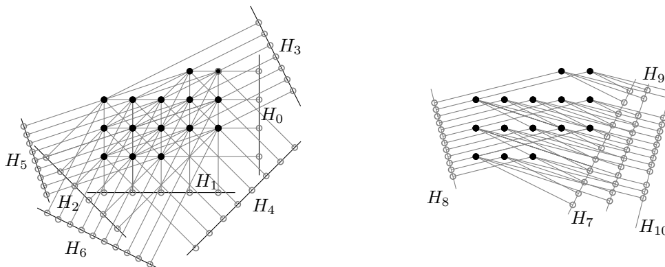
Fig. 7. A (4, 12) set of ghost chimneys.
