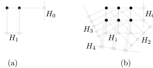
Fig. 5. Point sets showing that (a) t(1) \geq 2 and (b) t(2) \geq 5 .
