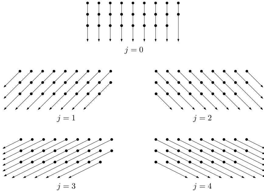
Fig. 3. The set S(i) for i = 9 and the projection directions that yield i, i + 1, \dots, i + 4 distinct points.
