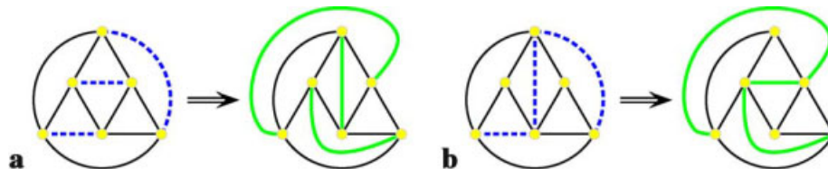
FIGURE 8. 3-edge flip in (a) the octahedron and (b) the other 6-vertex triangulation.
