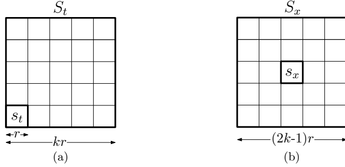
Fig. 1. (a) The square S_t has s_t on its left bottom corner. (b) The square S_x which is centered at s_x .
