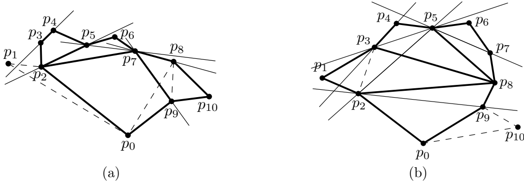
Figure 8: The sequence +- - + - + - + where p_1 is above l_{3,4} , p_6 is below l_{2,5} , p_8 is below l_{5,7} , and p_{10} is below l_{7,8} and above l_{7,9} . (b) The sequence +- - + - - - + where p_1 is above l_{3,4} and l_{2,9} and below l_{3,5} , p_6 is below l_{3,5} and l_{3,5} , and p_4 is below l_{5,7} .
