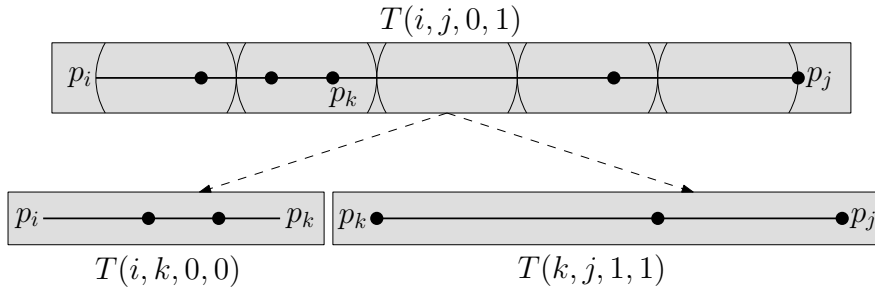
Figure 7: An instance for which the unit-disk covering (shown on the top interval) is not valid.
