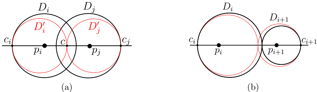
Figure 5: Illustrations of the proofs of (a) Lemma 5, and (b) Lemma 6.
